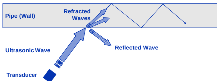
Figure 6.5. Ultrasonic Shear Wave
