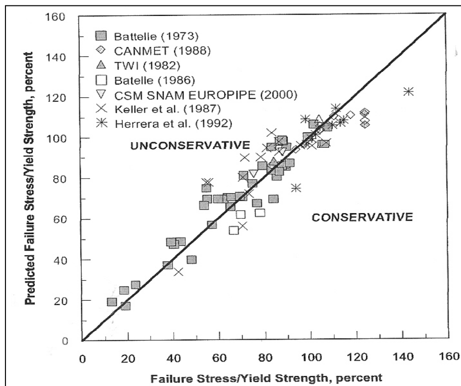
Figure 7.14 – Predictions of the Failure Pressure of Axially Oriented Gouges Using the NG-18 Equation (Cosham and Hopkins, 2002)
