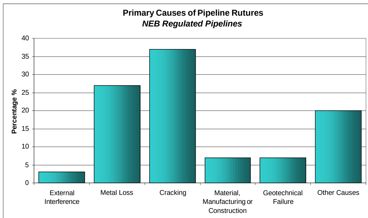
Figure 4.10 – Primary Causes of Pipeline Ruptures on NEB Regulated Pipeline (NEB, 2008)
