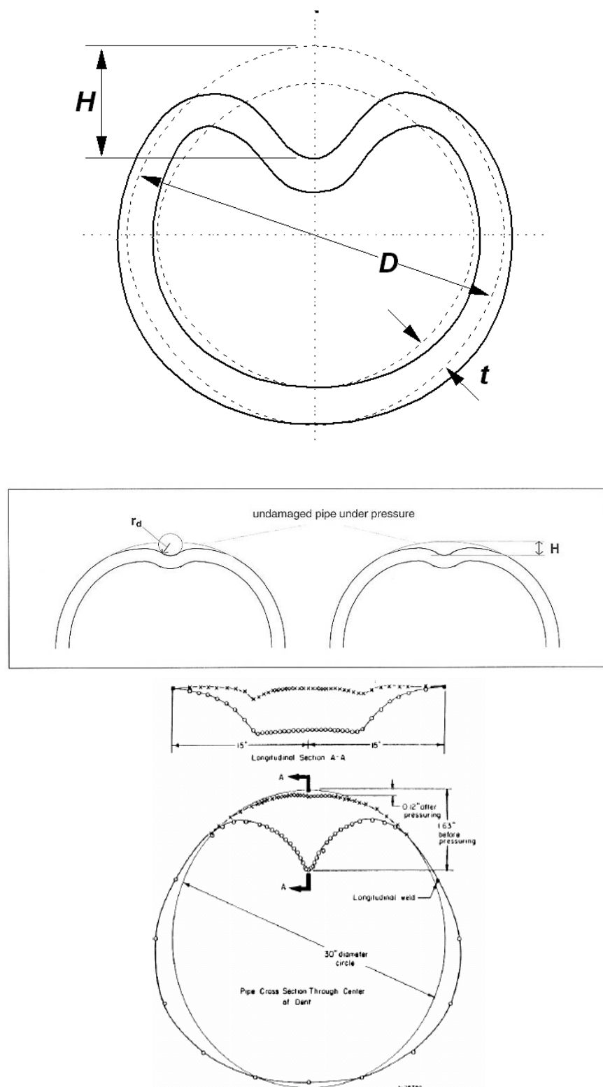
Figure 4.3 – Dent Depth Measurement (Hopkins and Leis, 2003)
