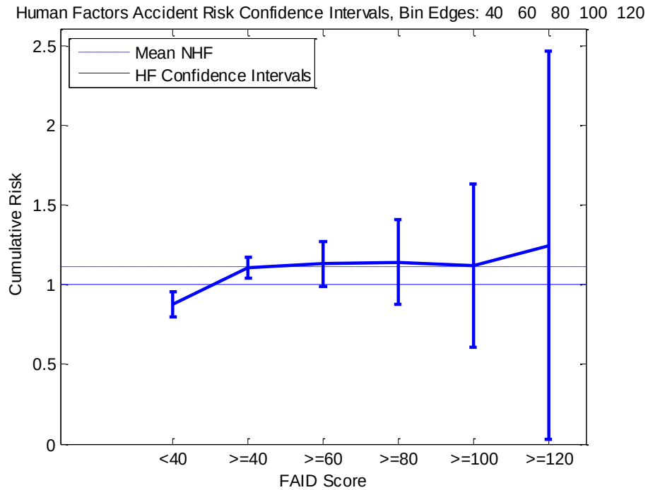
Figure 4. Confidence Intervals of Cumulative Risk for HF Accidents with Bin Anchors 40 and 120
