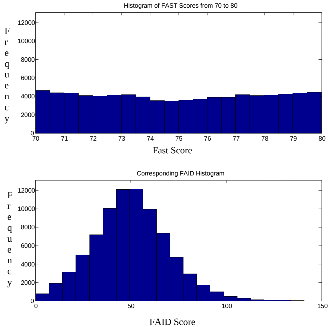
Figure 6. Distribution of FAST and FAID Scores Corresponding to FAST Bin of 70 to \leq 80
