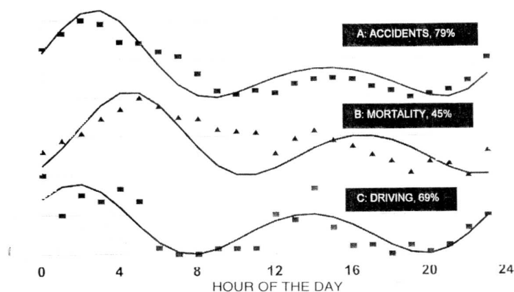
Figure 1. Curve fits to (A) accident (Mitler et al., 1988) and (B) mortality data (Mitler et al., 1988) and to (C) driver drowsiness data (Prokop & Prokop, 1955), with percentage variance explained for each curve fit. Curve parameter values are shown in the table below.
