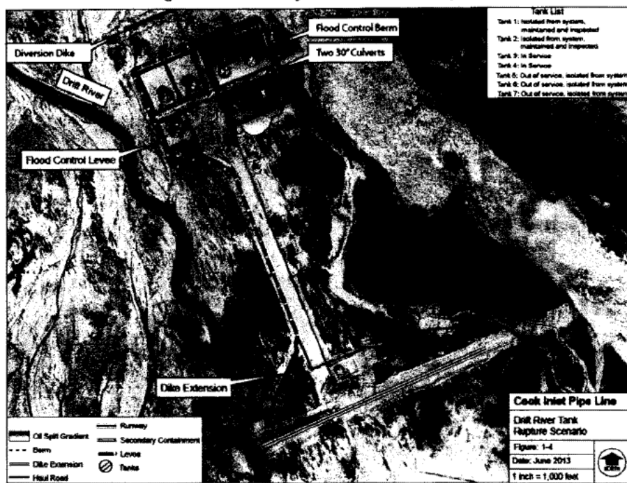
Figure 1-4: General Layout – Tanks 3 and 4 Rupture
