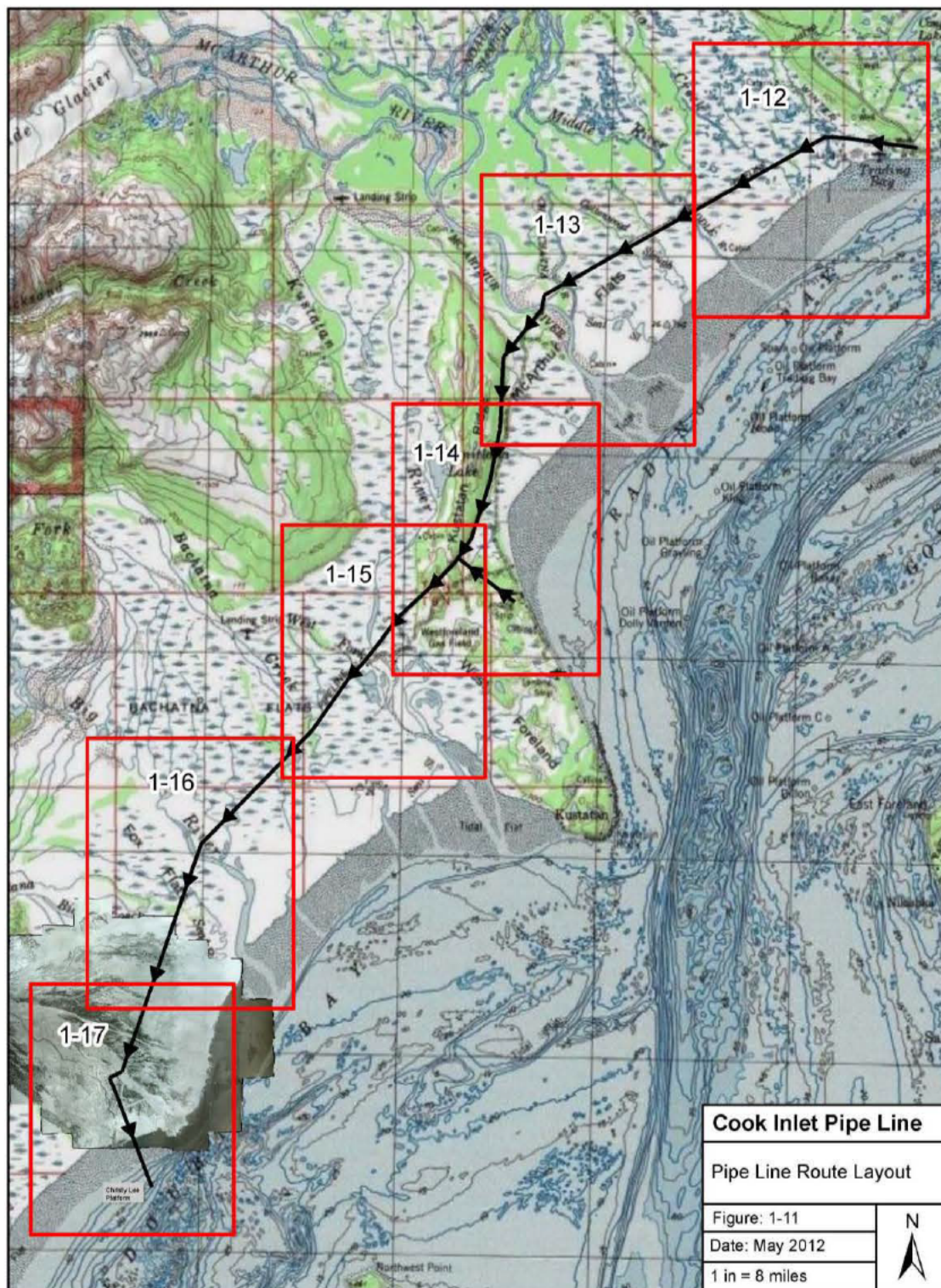
FIGURE 1-11: PIPE LINE ROUTE OVERVIEW DIAGRAM
